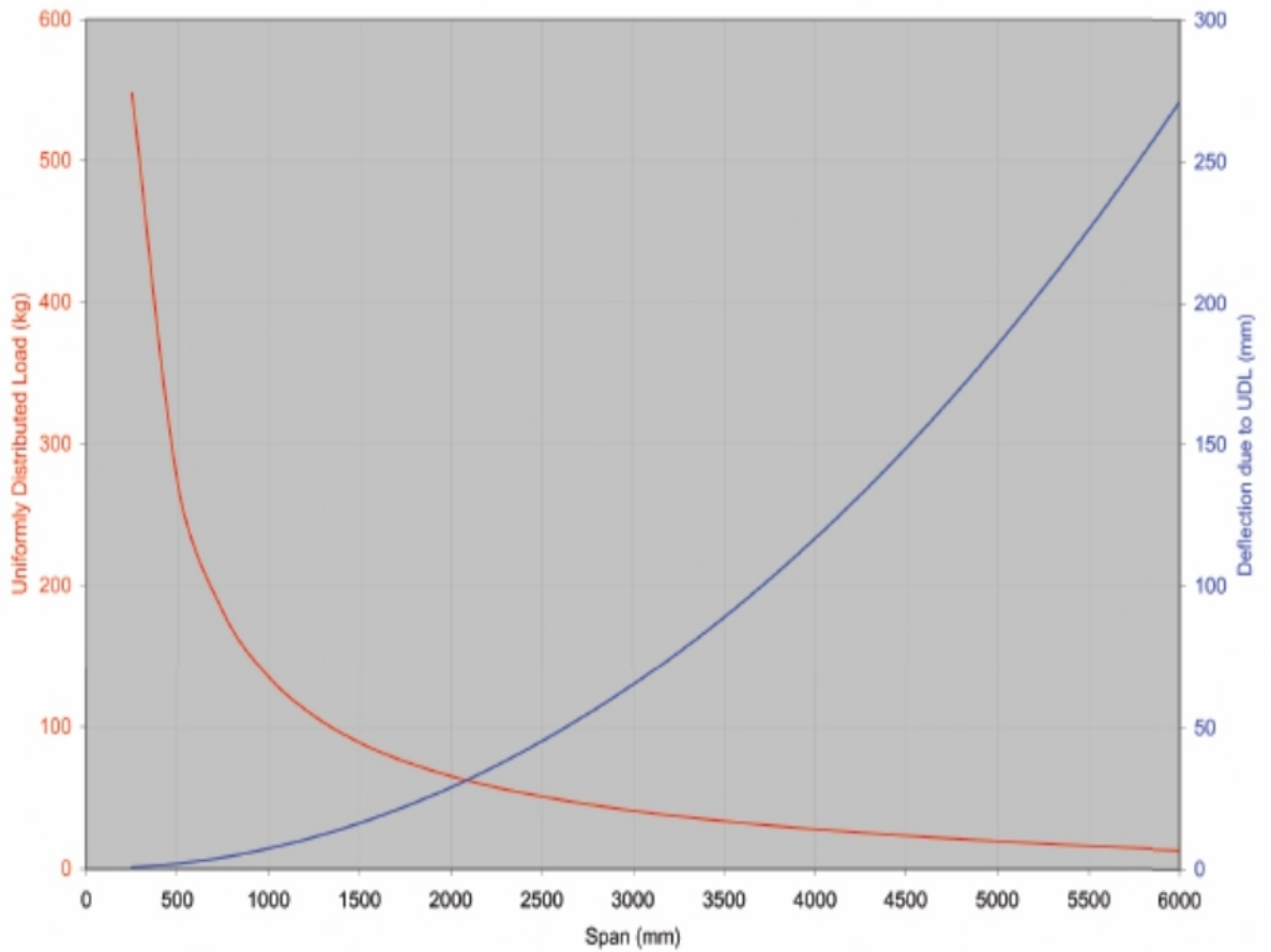
Load, Span & Deflection Graph
